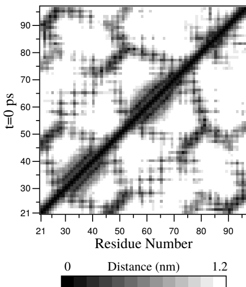
Fig. 6.55: A minimum distance matrix for a peptide 168 (page 543).
