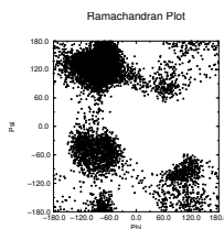
Fig. 6.60: Ramachandran plot of a small protein.
