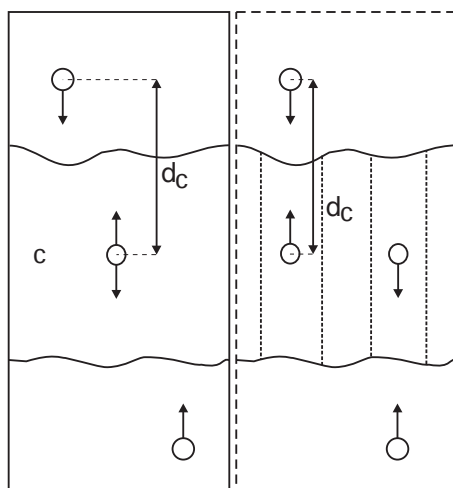
Fig. 6.36: Comparison of a plain center of mass reference group versus a cylinder reference group applied to interface systems. C is the reference group. The circles represent the center of mass of two groups plus the reference group, d_c is the reference distance.
