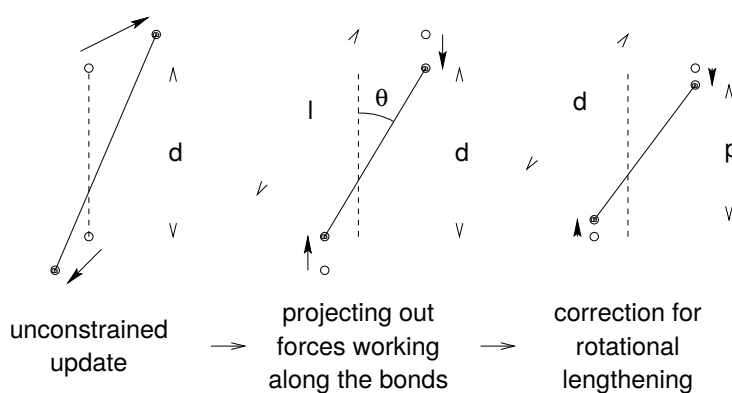
Fig. 6.8: The three position updates needed for one time step. The dashed line is the old bond of length d , the solid lines are the new bonds. l = d \cos \theta and p = (2d^2 - l^2)^{\frac{1}{2}} .
