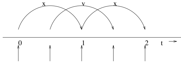
Fig. 6.7: The Leap-Frog integration method. The algorithm is called Leap-Frog because \mathbf{r} and \mathbf{v} are leaping like frogs over each other's backs.
