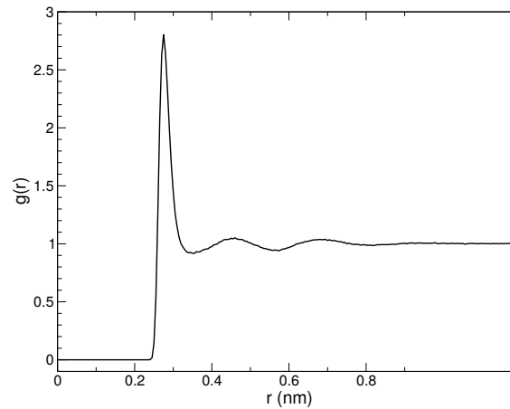
Fig. 6.51: g_{OO}(r) for Oxygen-Oxygen of SPC-water.
