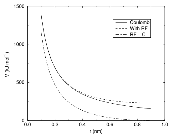
Fig. 6.17: The Coulomb interaction (for particles with equal signed charge) with and without reaction field. In the latter case \epsilon_r was 1, \epsilon_{rf} was 78, and r_c was 0.9 nm. The dot-dashed line is the same as the dashed line, except for a constant.
