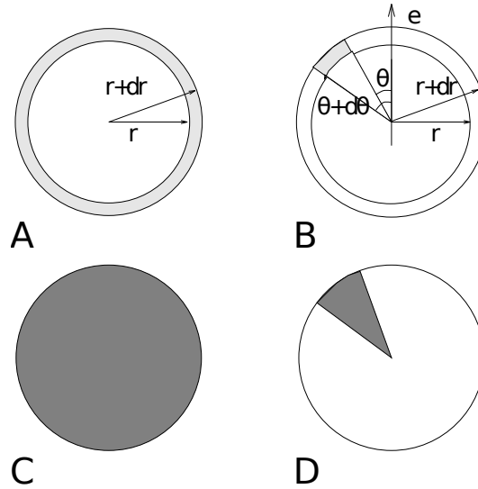
Fig. 6.50: Definition of slices in gmx rdf (page 188): A. g_{AB}(r) . B. g_{AB}(r, \theta) . The slices are colored gray. C. Normalization \langle \rho_B \rangle_{local} . D. Normalization \langle \rho_B \rangle_{local, \theta} . Normalization volumes are colored gray.
