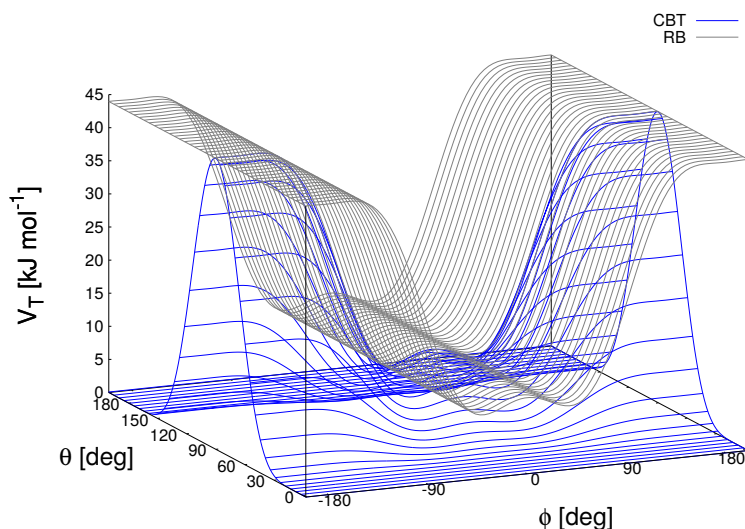
Fig. 6.27: Blue: surface plot of the combined bending-torsion potential ((6.52) with k = 10 \text{ kJ mol}^{-1} , a_0 = 2.41 , a_1 = -2.95 , a_2 = 0.36 , a_3 = 1.33 ) when, for simplicity, the bending angles behave the same ( \theta_1 = \theta_2 = \theta ). Gray: the same torsion potential without the \sin^3 \theta terms (Ryckaert-Bellemans type). \phi is the dihedral angle.
