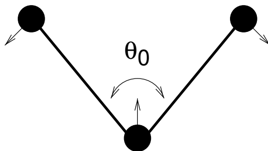
Fig. 6.20: Principle of angle vibration (left) and the bond angle potential (right).
