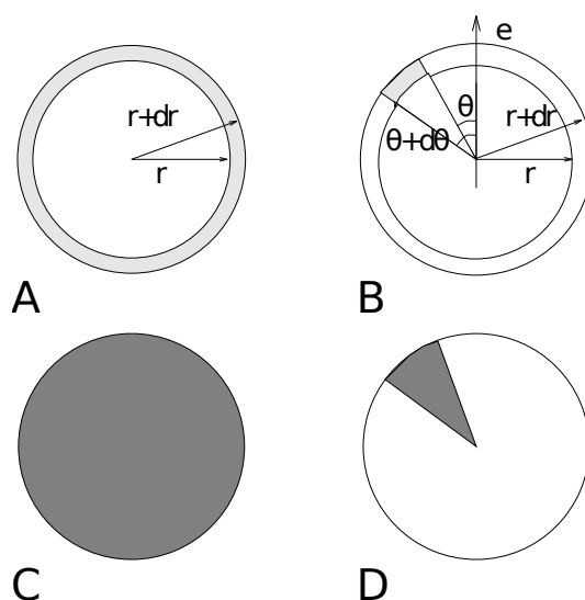
Fig. 5.50: Definition of slices in gmx rdf (page 134): A. g_{AB}(r) . B. g_{AB}(r, \theta) . The slices are colored gray. C. Normalization \langle \rho_B \rangle_{local} . D. Normalization \langle \rho_B \rangle_{local, \theta} . Normalization volumes are colored gray.
