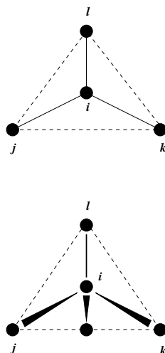
Fig. 5.23: Principle of improper dihedral angles. Out of tetrahedral angle. The improper dihedral angle \xi is defined as the angle between planes (i,j,k) and (j,k,l) .
