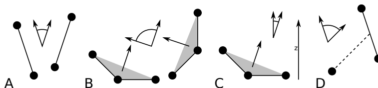
Fig. 5.54: Angle options of gmx gangle (page 90): A. Angle between two vectors. B. Angle between two planes. C. Angle between a vector and the z axis. D. Angle between a vector and the normal of a sphere. Also other combinations are supported: planes and vectors can be used interchangeably.
