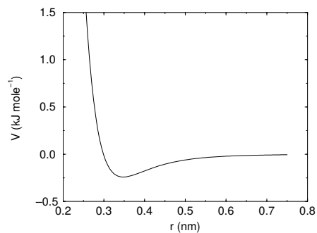
Fig. 5.16: The Buckingham interaction.
