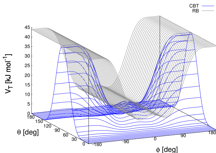
Fig. 5.27: Blue: surface plot of the combined bending-torsion potential ((5.179) with k = 10 \text{ kJ mol}^{-1} , a_0 = 2.41 , a_1 = -2.95 , a_2 = 0.36 , a_3 = 1.33 ) when, for simplicity, the bending angles behave the same ( \theta_1 = \theta_2 = \theta ). Gray: the same torsion potential without the \sin^3 \theta terms (Ryckaert-Bellemans type). \phi is the dihedral angle.
