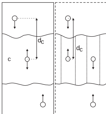
Fig. 5.37: Comparison of a plain center of mass reference group versus a cylinder reference group applied to interface systems. C is the reference group. The circles represent the center of mass of two groups plus the reference group, d_c is the reference distance.
