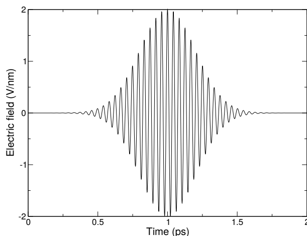
Fig. 5.46: A simulated laser pulse in GROMACS.
