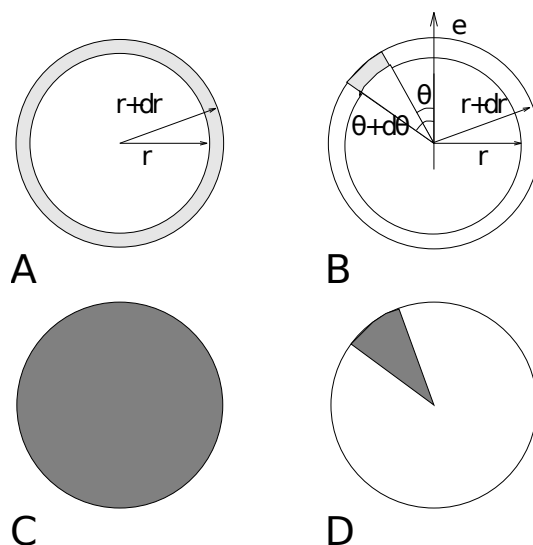
Fig. 5.52: Definition of slices in gmx rdf (page 135): A. g_{AB}(r) . B. g_{AB}(r, \theta) . The slices are colored gray. C. Normalization \langle \rho_B \rangle_{local} . D. Normalization \langle \rho_B \rangle_{local, \theta} . Normalization volumes are colored gray.
