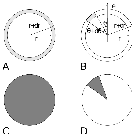
Fig. 5.52: Definition of slices in gmx rdf (page 229): A. g_{AB}(r) . B. g_{AB}(r, \theta) . The slices are colored gray. C. Normalization \langle \rho_B \rangle_{local} . D. Normalization \langle \rho_B \rangle_{local, \theta} . Normalization volumes are colored gray.
