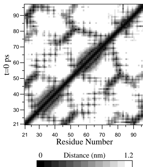
Figure 8.7: A minimum distance matrix for a peptide [153].
