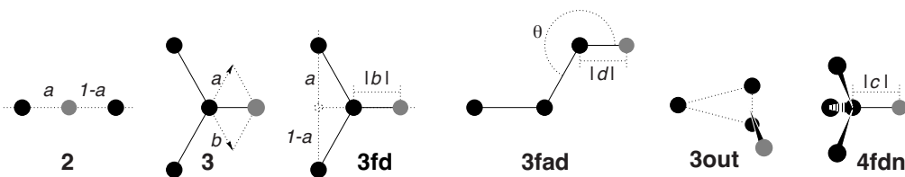
Figure 4.19: The six different types of virtual site construction in GROMACS. The constructing atoms are shown as black circles, the virtual sites in gray.
