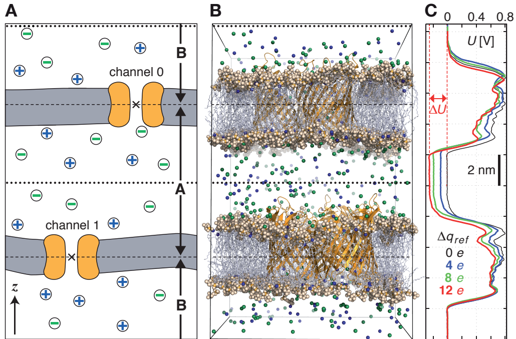
Figure 6.7: Typical double-membrane setup for CompEL simulations (A, B). Plot (C) shows the potential difference \Delta U resulting from the selected charge imbalance \Delta q_{ref} between the compartments.
