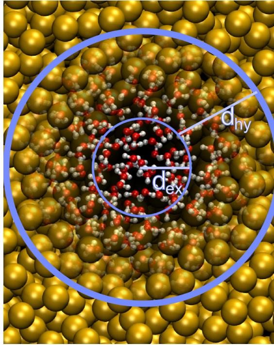
Figure 6.10: A schematic illustration of the AdResS method for water.
