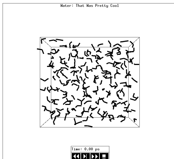
Fig. 6.49: The window of gmx view (page 227) showing a box of water.
