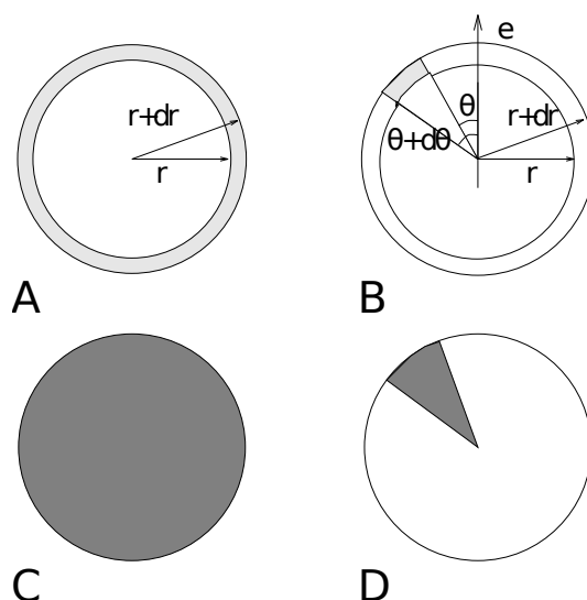
Fig. 6.50: Definition of slices in gmx rdf (page 189): A. g_{AB}(r) . B. g_{AB}(r, \theta) . The slices are colored gray. C. Normalization \langle \rho_B \rangle_{local} . D. Normalization \langle \rho_B \rangle_{local, \theta} . Normalization volumes are colored gray.
