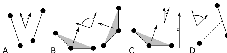
Fig. 6.54: Angle options of gmx gangle (page 146): A. Angle between two vectors. B. Angle between two planes. C. Angle between a vector and the z axis. D. Angle between a vector and the normal of a sphere. Also other combinations are supported: planes and vectors can be used interchangeably.
