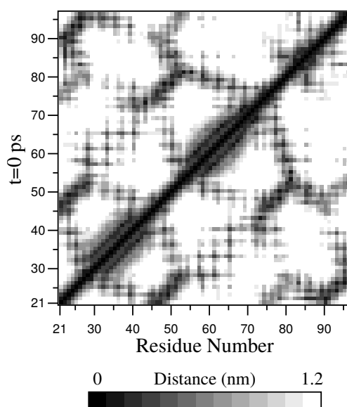
Fig. 5.55: A minimum distance matrix for a peptide 168 (page 519).
