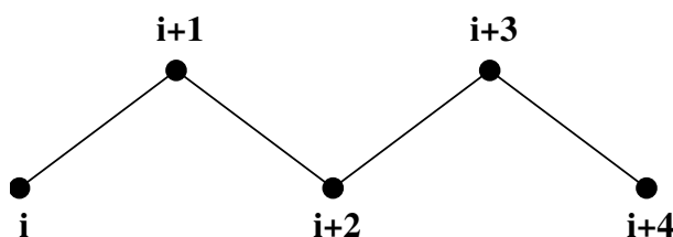
Fig. 5.33: Atoms along an alkane chain.
