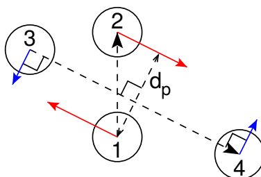
Fig. 5.38: The pull setup for geometry direction-relative . The “normal” pull groups are 1 and 2. Groups 3 and 4 define the pull direction and thus the direction of the normal pull forces (red). This leads to reaction forces (blue) on groups 3 and 4, which are perpendicular to the pull direction. Their magnitude is given by the “normal” pull force times the ratio of d_p and the distance between groups 3 and 4.
