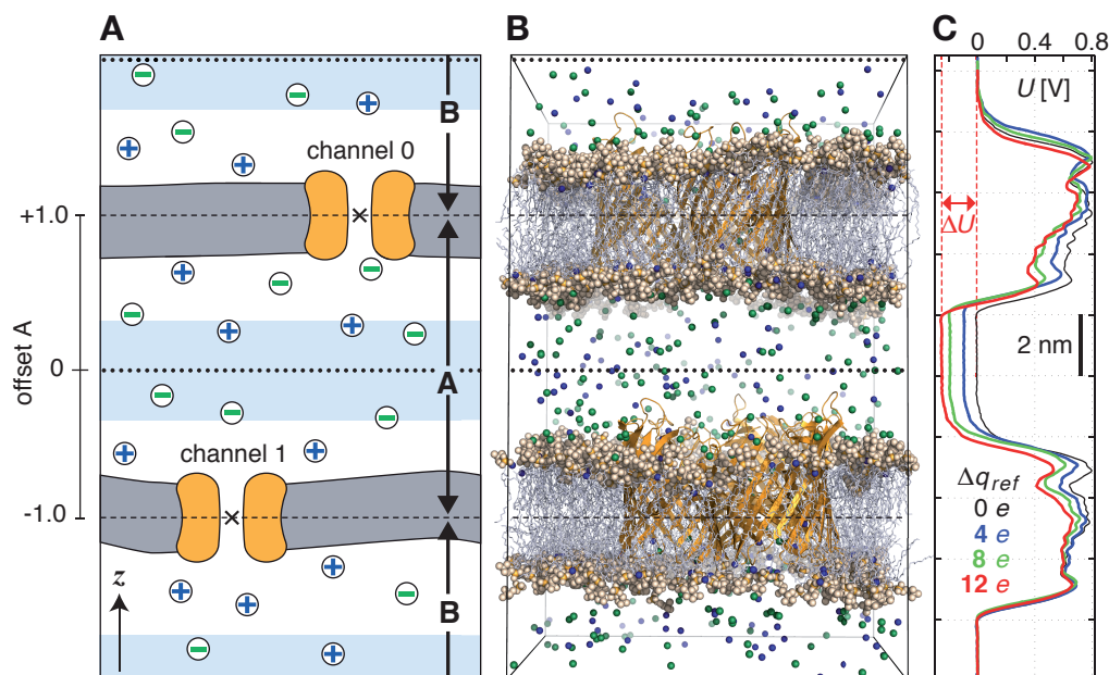
Fig. 5.47: Typical double-membrane setup for CompEL simulations (A, B). Ion/water molecule exchanges will be performed as needed between the two light blue volumes around the dotted black lines (A). Plot (C) shows the potential difference \Delta U resulting from the selected charge imbalance \Delta q_{ref} between the compartments.
