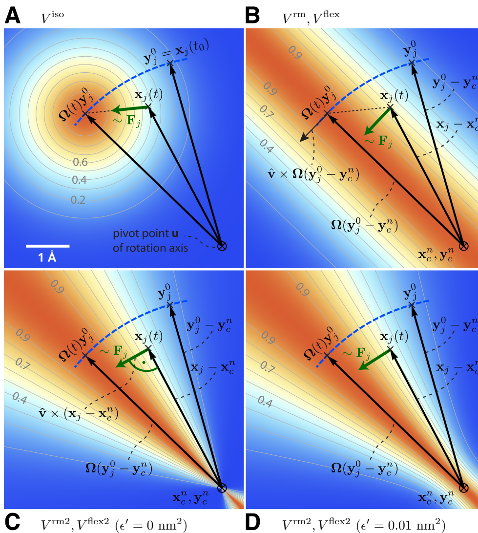
Fig. 5.44: Selection of different rotation potentials and definition of notation. All four potentials V (color coded) are shown for a single atom at position \mathbf{x}_j(t) . A: Isotropic potential V^{\text{iso}} , B: radial motion potential V^{\text{rm}} and flexible potential V^{\text{flex}} , C–D: radial motion2 potential V^{\text{rm}2} and flexible2 potential V^{\text{flex}2} for \epsilon' = 0 \text{ nm}^2 (C) and \epsilon' = 0.01 \text{ nm}^2 (D). The rotation axis is perpendicular to the plane and marked by \otimes . The light gray contours indicate Boltzmann factors e^{-V/(k_B T)} in the \mathbf{x}_j -plane for T = 300 \text{ K} and k = 200 \text{ kJ}/(\text{mol} \cdot \text{nm}^2) . The green arrow shows the direction of the force \mathbf{F}_j acting on atom j ; the blue dashed line indicates the motion of the reference position.
