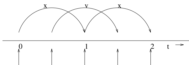
Fig. 5.7: The Leap-Frog integration method. The algorithm is called Leap-Frog because \mathbf{r} and \mathbf{v} are leaping like frogs over each other's backs.
