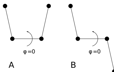
Fig. 5.54: Dihedral conventions: A. “Biochemical convention”. B. “Polymer convention”.
