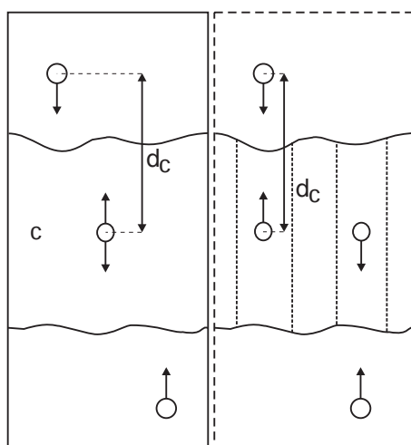
Fig. 5.37: Comparison of a plain center of mass reference group versus a cylinder reference group applied to interface systems. C is the reference group. The circles represent the center of mass of two groups plus the reference group, d_c is the reference distance.
