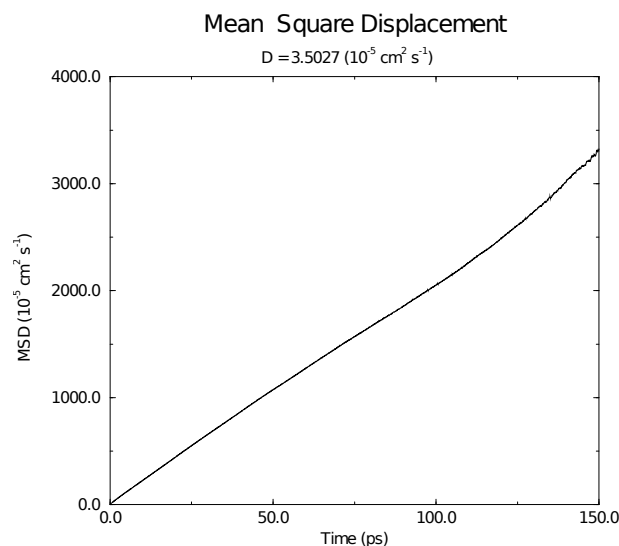
Fig. 5.53: Mean Square Displacement of SPC-water.
