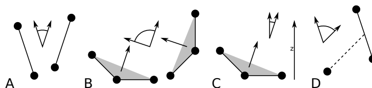
Fig. 5.55: Angle options of gmx gangle (page 90): A. Angle between two vectors. B. Angle between two planes. C. Angle between a vector and the z axis. D. Angle between a vector and the normal of a sphere. Also other combinations are supported: planes and vectors can be used interchangeably.
