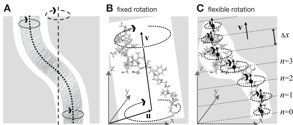
Fig. 5.43: Comparison of fixed and flexible axis rotation. A: Rotating the sketched shape inside the white tubular cavity can create artifacts when a fixed rotation axis (dashed) is used. More realistically, the shape would revolve like a flexible pipe-cleaner (dotted) inside the bearing (gray). B: Fixed rotation around an axis \mathbf{v} with a pivot point specified by the vector \mathbf{u} . C: Subdividing the rotating fragment into slabs with separate rotation axes ( \uparrow ) and pivot points ( \bullet ) for each slab allows for flexibility. The distance between two slabs with indices n and n + 1 is \Delta x .
