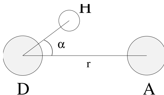
Fig. 5.57: Geometrical Hydrogen bond criterion.
