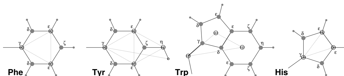
Fig. 5.49: The different types of virtual site constructions used for aromatic residues. The atoms used in the construction of the virtual site(s) are depicted as black circles, virtual sites as gray ones. Hydrogens are smaller than heavy atoms. A: phenylalanine; B: tyrosine (note that the hydroxyl hydrogen is not a virtual site); C: tryptophan; D: histidine.
