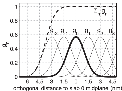
Fig. 5.45: Gaussian functions g_n centered at n \Delta x for a slab distance \Delta x = 1.5 nm and n \geq -2 . Gaussian function g_0 is highlighted in bold; the dashed line depicts the sum of the shown Gaussian functions.
