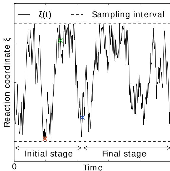
Fig. 5.39: AWH evolution in time for a Brownian particle in a double-well potential. The reaction coordinate \xi(t) traverses the sampling interval multiple times in the initial stage before exiting and entering the final stage. In the final stage, the dynamics of \xi becomes increasingly diffusive.
