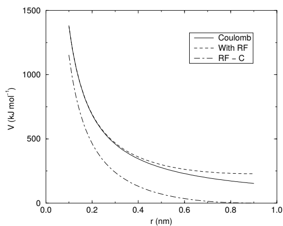
Fig. 5.18: The Coulomb interaction (for particles with equal signed charge) with and without reaction field. In the latter case \epsilon_r was 1, \epsilon_{rf} was 78, and r_c was 0.9 nm. The dot-dashed line is the same as the dashed line, except for a constant.
