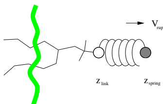
Fig. 5.36: Schematic picture of pulling a lipid out of a lipid bilayer with umbrella pulling. V_{rup} is the velocity at which the spring is retracted, Z_{link} is the atom to which the spring is attached and Z_{spring} is the location of the spring.
