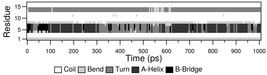
Fig. 5.61: Analysis of the secondary structure elements of a peptide in time.
