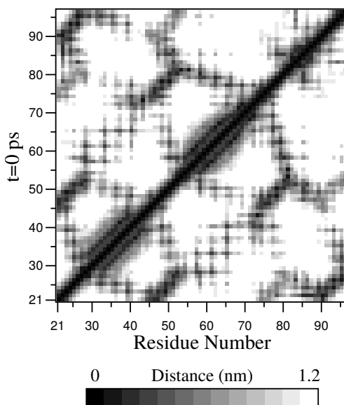
Fig. 5.58: A minimum distance matrix for a peptide 168 (page 542).
