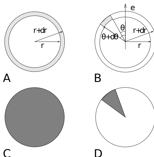
Fig. 5.53: Definition of slices in gmx rdf (page 209): A. g_{AB}(r) . B. g_{AB}(r, \theta) . The slices are colored gray. C. Normalization \langle \rho_B \rangle_{local} . D. Normalization \langle \rho_B \rangle_{local, \theta} . Normalization volumes are colored gray.
